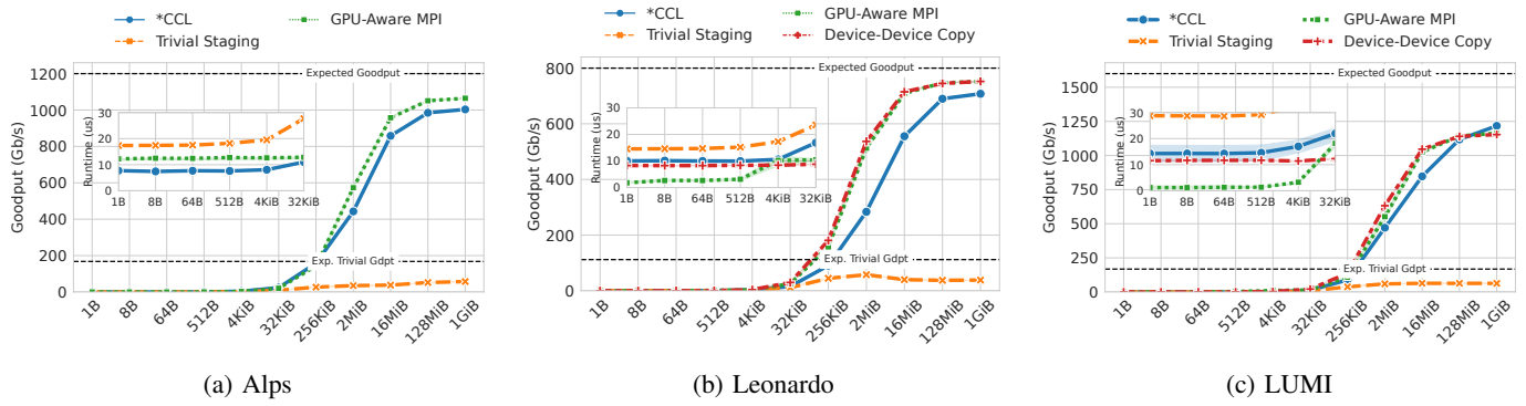
Fig. 3: GPU-GPU unidirectional transfers performance. For the sake of readability, we use different y-axis ranges.
