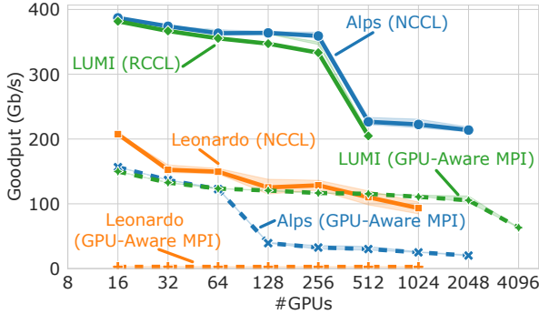
Fig. 10: 1 GiB allreduce scalability.
